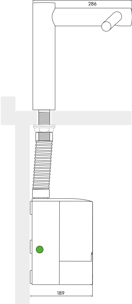
SIDE ELEVATION
